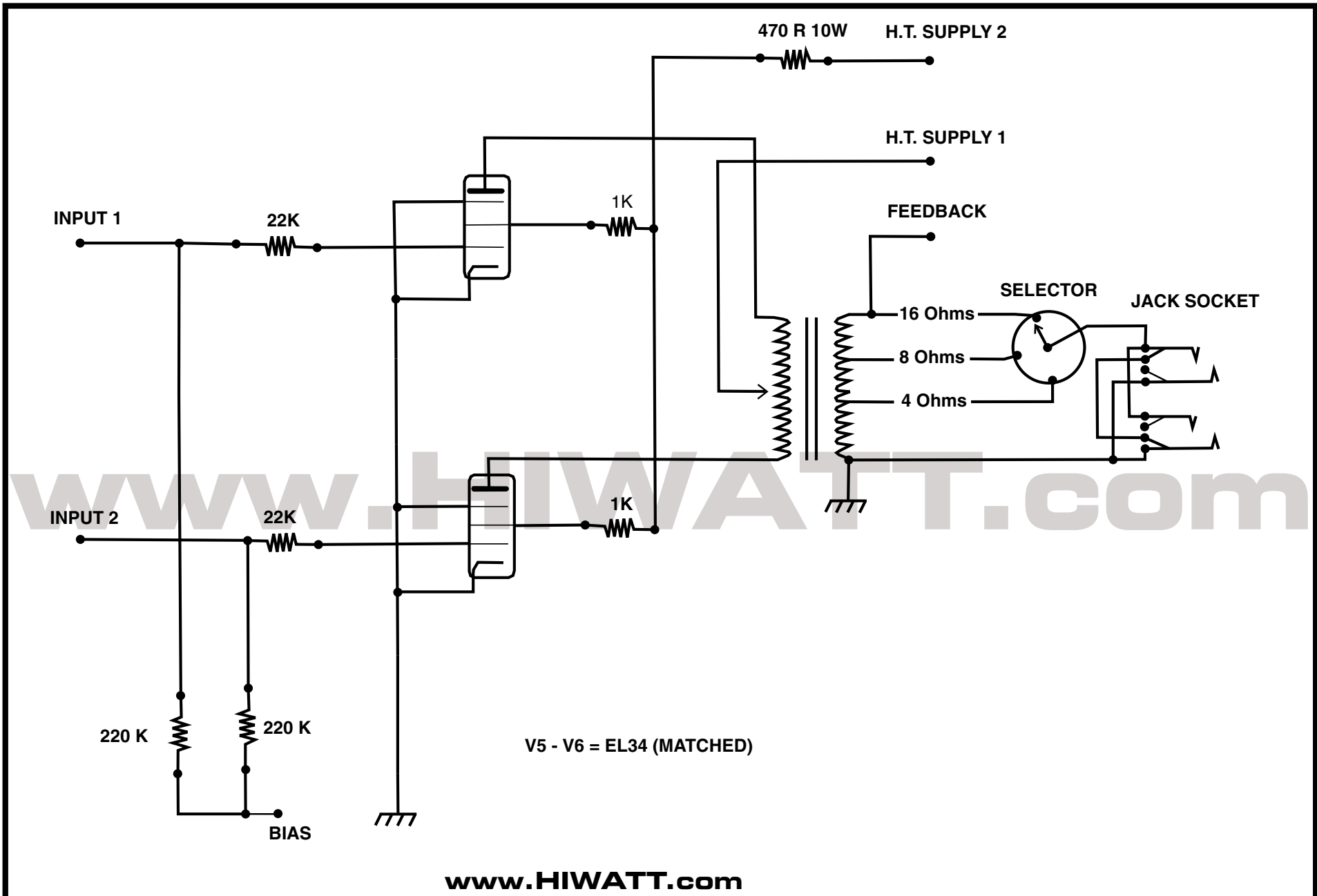
HIWATT® DR504 OUTPUT STAGE CIRCUIT DIAGRAM Copyright © HIWATT Amplification 2001
